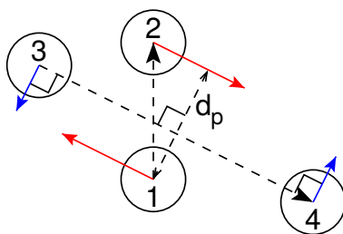
Fig. 5.39: The pull setup for geometry direction-relative . The “normal” pull groups are 1 and 2. Groups 3 and 4 define the pull direction and thus the direction of the normal pull forces (red). This leads to reaction forces (blue) on groups 3 and 4, which are perpendicular to the pull direction. Their magnitude is given by the “normal” pull force times the ratio of d_p and the distance between groups 3 and 4.
