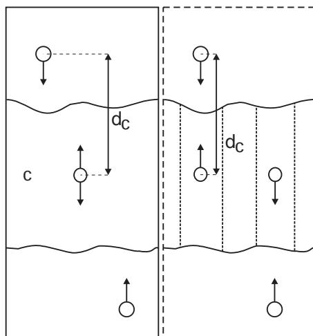
Fig. 5.38: Comparison of a plain center of mass reference group versus a cylinder reference group applied to interface systems. C is the reference group. The circles represent the center of mass of two groups plus the reference group, d_c is the reference distance.
