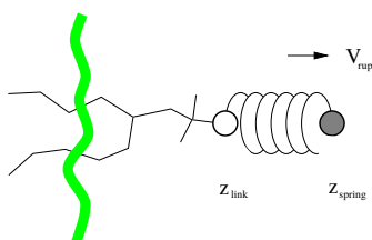
Fig. 5.37: Schematic picture of pulling a lipid out of a lipid bilayer with umbrella pulling. V_{rup} is the velocity at which the spring is retracted, Z_{link} is the atom to which the spring is attached and Z_{spring} is the location of the spring.
