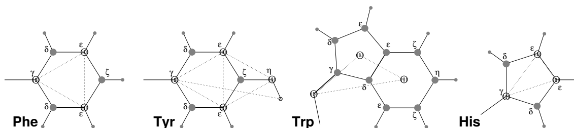
Fig. 5.50: The different types of virtual site constructions used for aromatic residues. The atoms used in the construction of the virtual site(s) are depicted as black circles, virtual sites as gray ones. Hydrogens are smaller than heavy atoms. A: phenylalanine; B: tyrosine (note that the hydroxyl hydrogen is not a virtual site); C: tryptophan; D: histidine.
