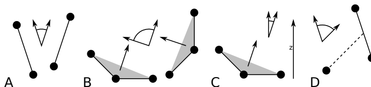
Fig. 5.56: Angle options of gmx gangle (page 90): A. Angle between two vectors. B. Angle between two planes. C. Angle between a vector and the z axis. D. Angle between a vector and the normal of a sphere. Also other combinations are supported: planes and vectors can be used interchangeably.
