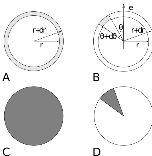
Fig. 5.52: Definition of slices in gmx rdf (page 135): A. g_{AB}(r) . B. g_{AB}(r, \theta) . The slices are colored gray. C. Normalization \langle \rho_B \rangle_{local} . D. Normalization \langle \rho_B \rangle_{local, \theta} . Normalization volumes are colored gray.
